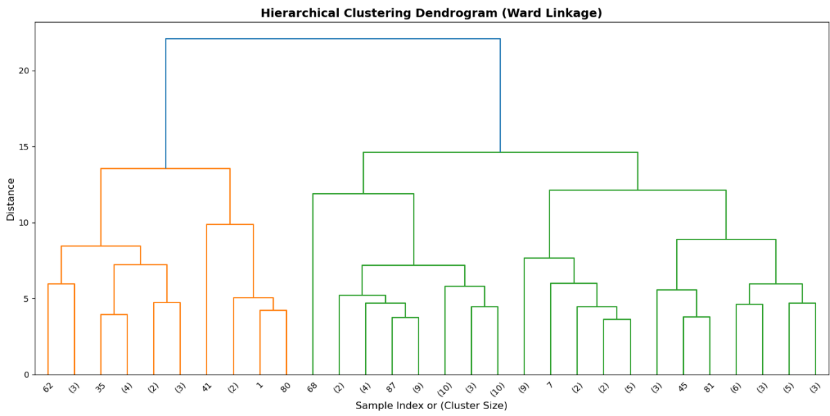
Figure 9. Hierarchical Clustering Dendrogram
