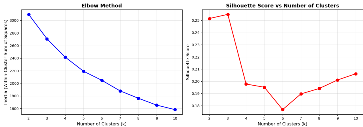
Figure 7. Elbow Method and Silhouette Scores for K-Means Clustering
