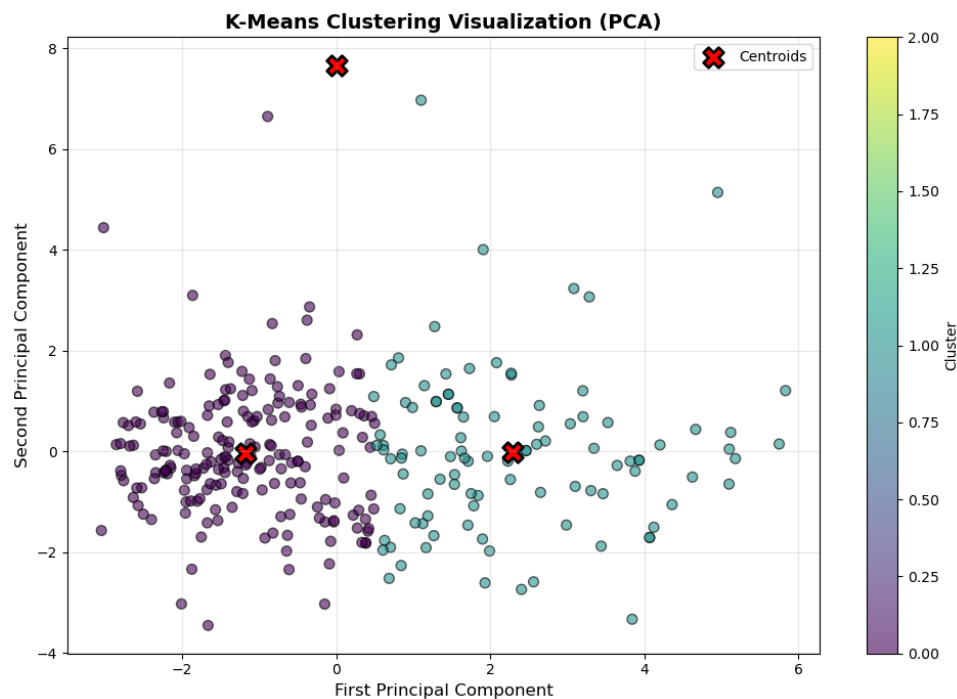
Figure 8. K-Means Clustering Visualization
