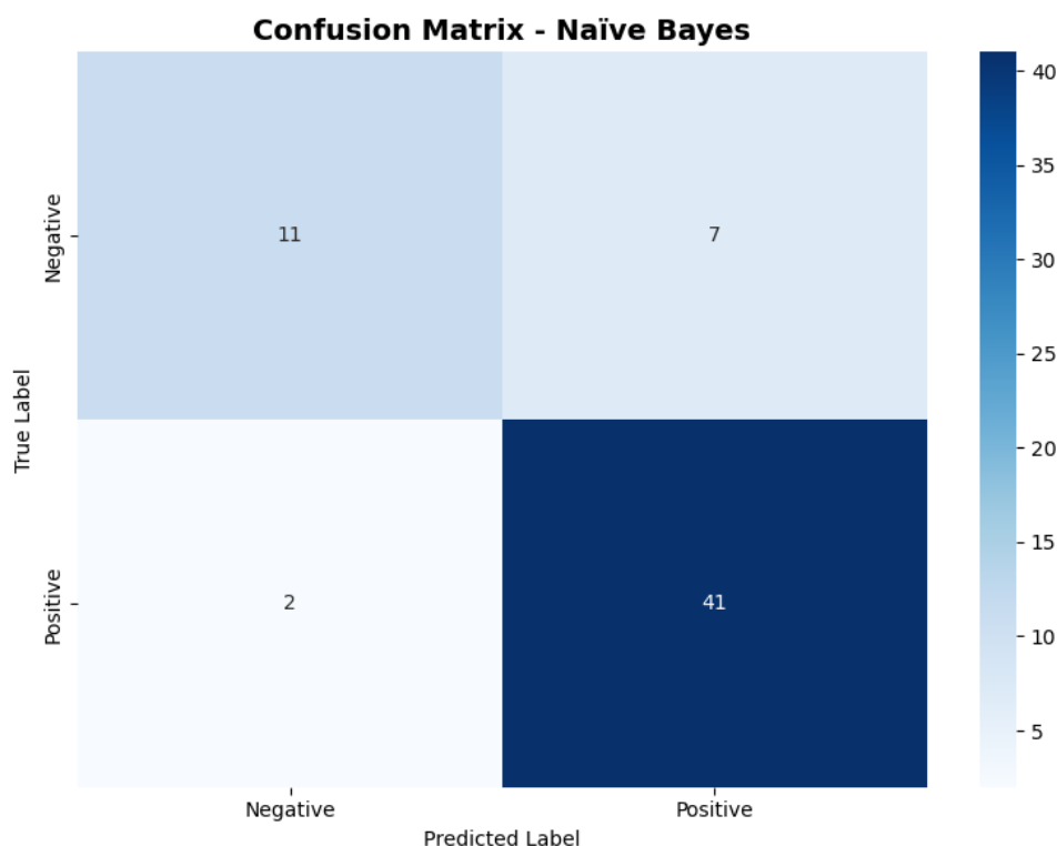
Figure 6. Confusion Matrix for Naïve Bayes Classification
