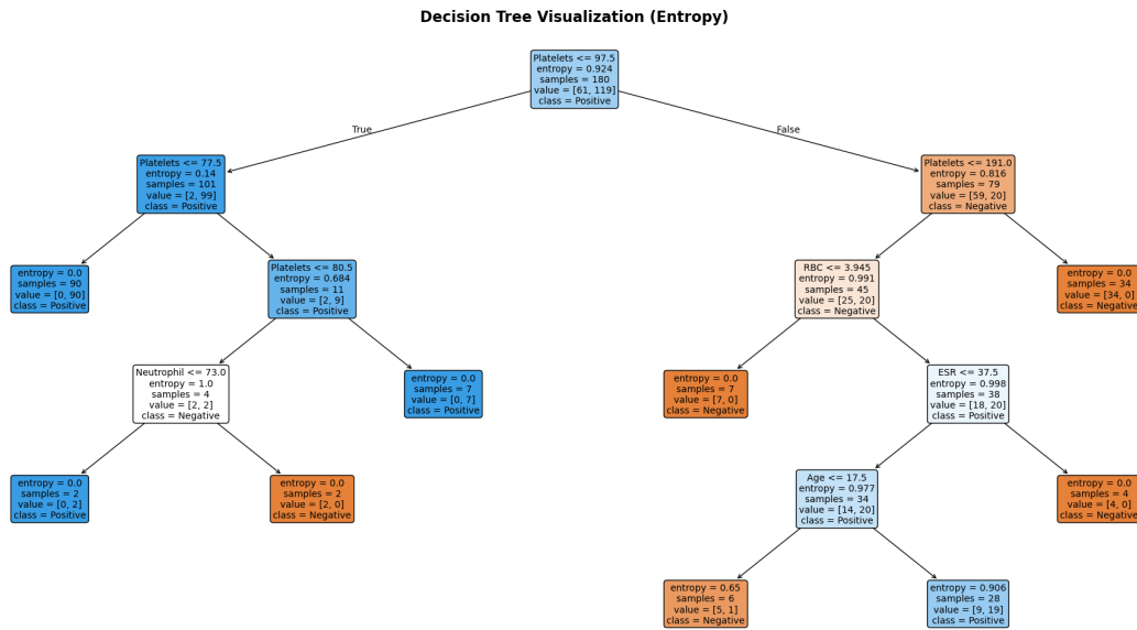
Figure 5. Decision Tree Visualization
